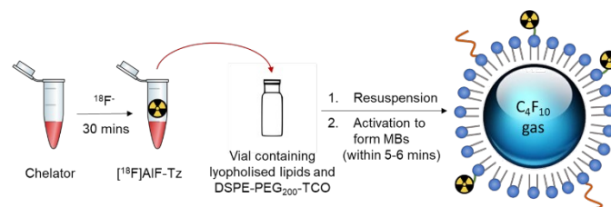
Figure 5: Development of a kit-based approach for ^{18}\text{F} -labelling of microbubbles.
