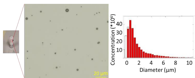
Figure 2: Left: Optical microscopy image of microbubbles; Right: Size distribution of microbubbles.
