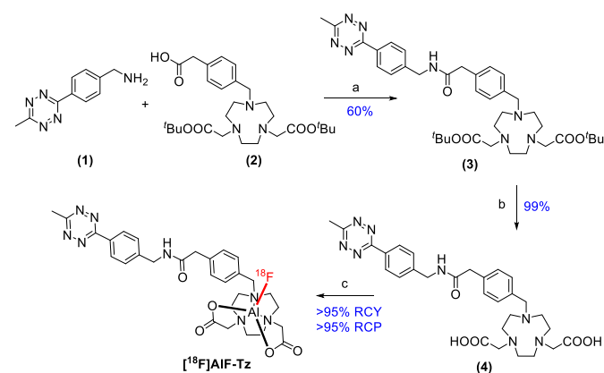
Scheme 1: Synthesis of ^{18}\text{F} ]AlF-Tz. Reaction conditions: a) HBTU, Et 3 N, DMF, 40 °C, 24 h; b) TFA, CH 2 Cl 2 , r.t., 24 h; c) AlCl 3 , ^{18}\text{F} ]-, 0.5 M sodium acetate:MeCN 2:3 v.v, pH 4.2, 100 °C, 20 min.
