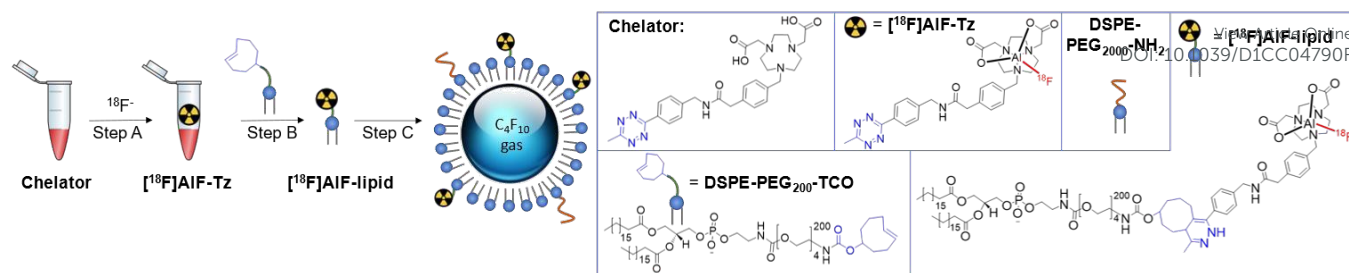
Figure 1: Schematic representation of ^{18}\text{F} -labelling of microbubbles developed in this study, where radiolabelling is achieved by reaction of a TCO-containing lipid (DSPE-PEG 2000 -TCO) and a tetrazine-functionalised ^{18}\text{F} prosthetic group. Step A: ^{18}\text{F} -labelling of chelator (>95% RCY, RCP); Step B: IEDDA reaction of ^{18}\text{F} -labelled chelator and TCO-lipid (40-50% RCY); Step C: Formation of ^{18}\text{F} ]AlF-microbubbles (40-50% RCY).
