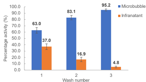
Figure 4: Comparison of activities of microbubble foam against infranatant after successive centrifuge washes. Reactions were performed in triplicate ( n=3 ), values presented as mean \pm SD.
